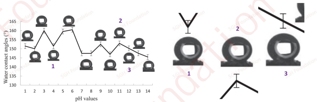
Fig. 18. Stability of fCGA-10 aerogel at different pH values.
