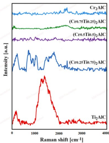
Fig. 12. Raman spectrum of each sample.
